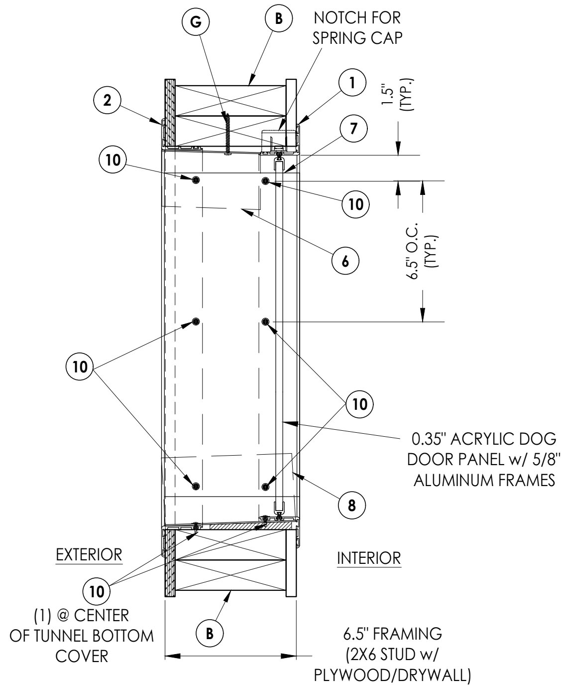
1 3 VERTICAL CROSS SECTION Shown w/ Large Size Dog Door 2X Stud Framing Installation
