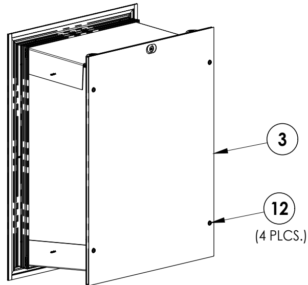
INTERIOR SECURITY COVER REQUIRED FOR DESIGN PRESSURE > 50 PSF
