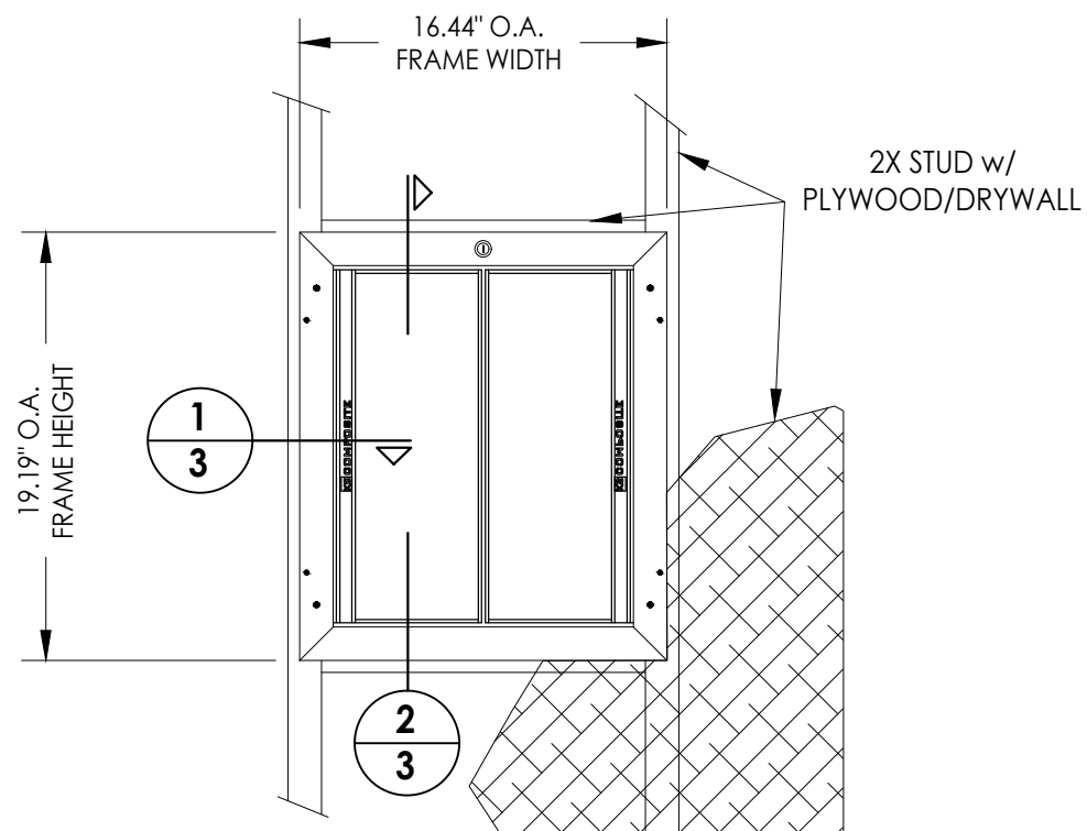
INTERIOR VIEW Large Size Dog Door Shown
