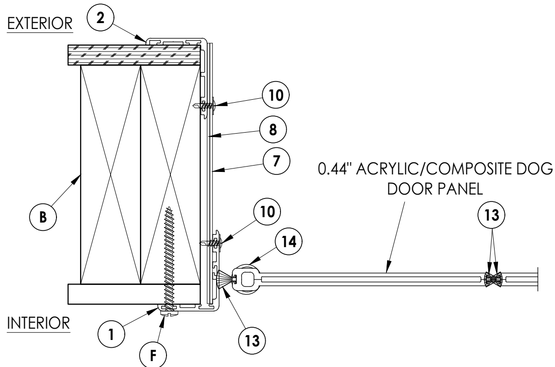
2 3 HORIZONTAL CROSS SECTION FOR PLEXIDOR SIZES LG & MD (UP TO 16.44" X 19.19")
