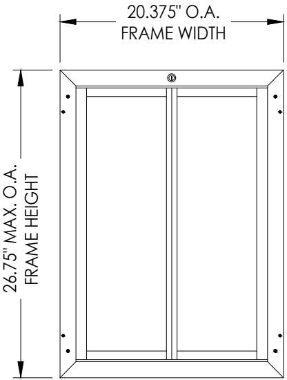
INTERIOR VIEW PD WALL MOUNT (X-LARGE)
