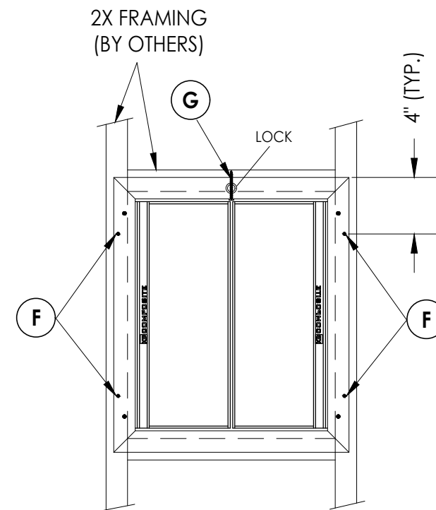
INTERIOR FRAME ANCHORING
