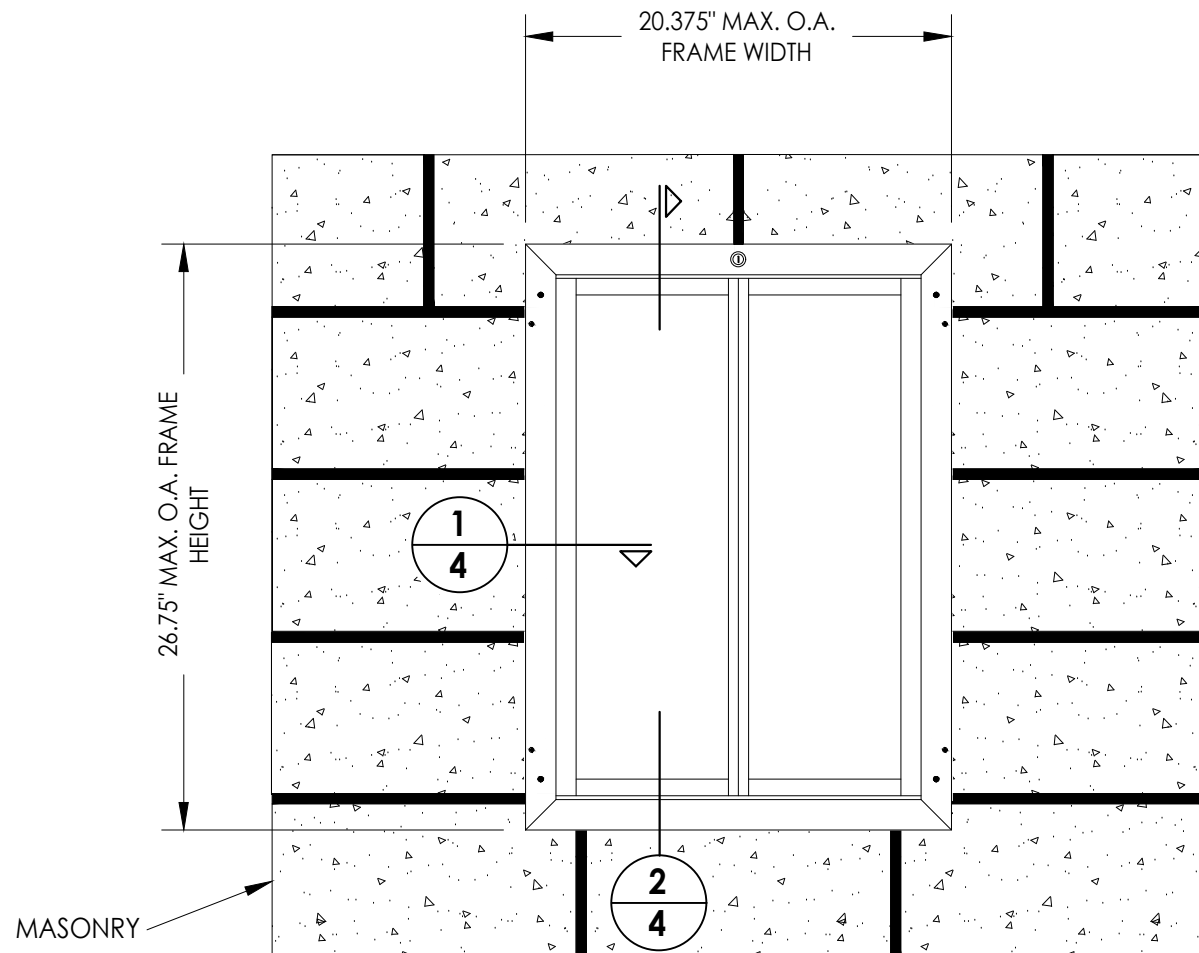
INTERIOR VIEW X-Large Size Dog Door Shown
